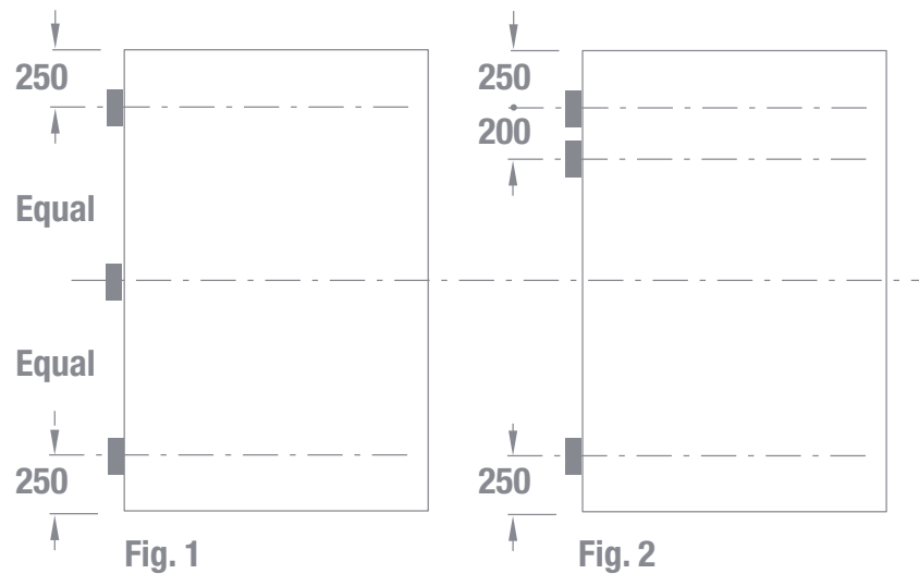
Doors up to 2,100mm height (3 hinges)
