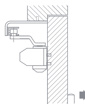
Parallel arm installation On push side
